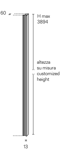
Profilo terminale Terminal profile
