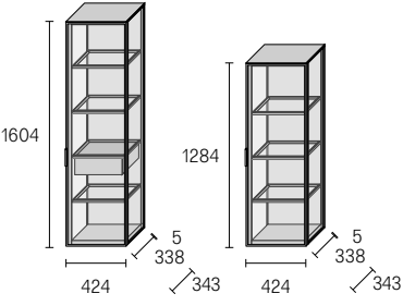
Alambra vetrina pensile con anta battente Alambra suspended cabinet with hinged door
