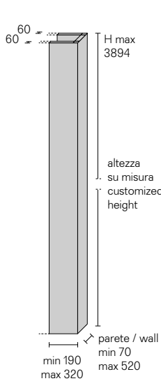
Terminale colonna C-shaped closing panel
